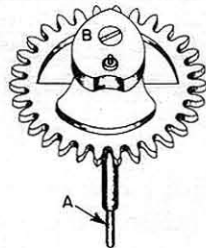
Minute Register Wheel Assembly No. 19
