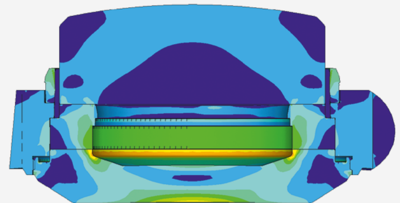
Computer model of the pressure exerted on the watch at 15,000 metres. The scale of stress levels ranges from near zero in blue to the maximum in red. The pressure on the crystal and on the case back, which is borne by the Ringlock compression ring, is shown in blue and green.
